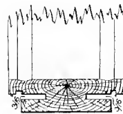
Fig. 2376. Section through Cover-strips.
